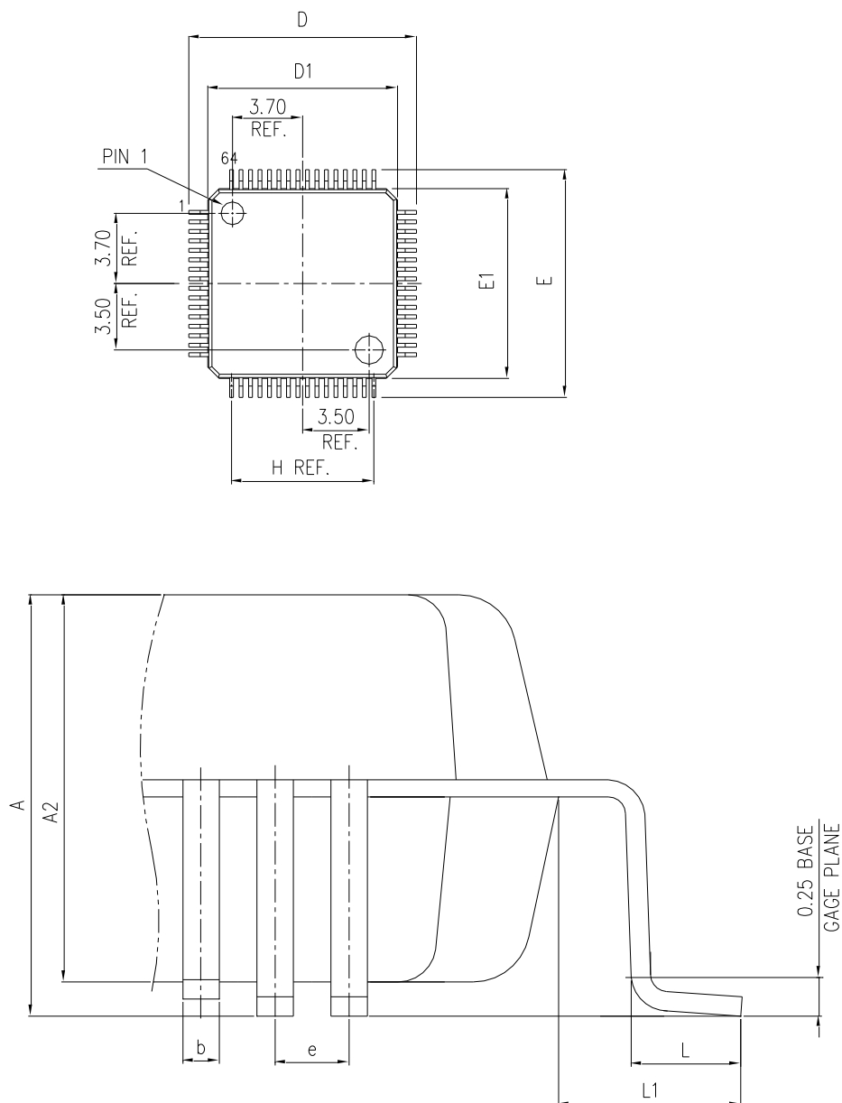
Figure 25 LQFP64 Package Diagram
